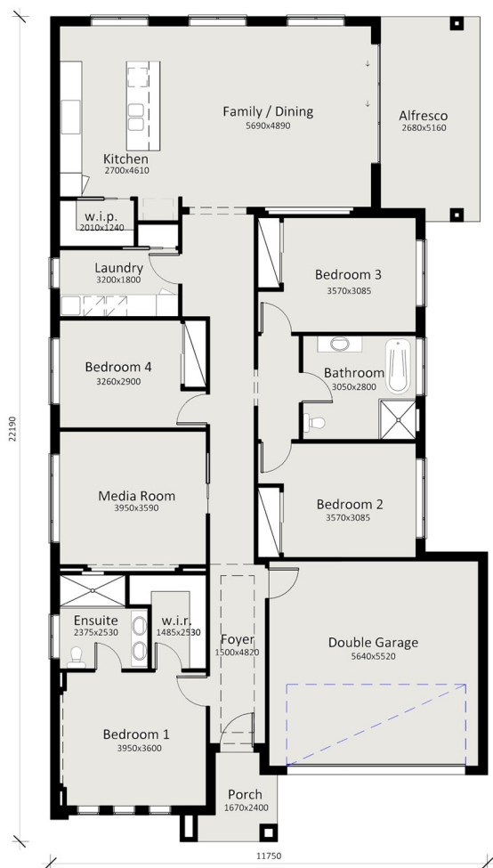
Floor Plan Scale 1 : 100
